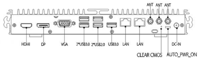
Rear Panel External I/O
